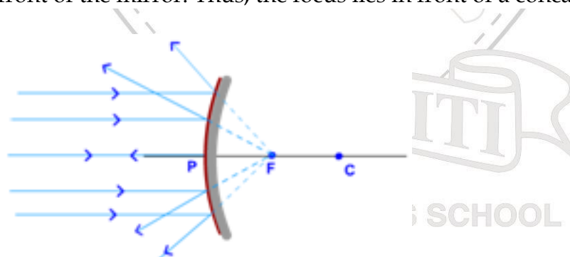
Fig: Diverging Mirror
