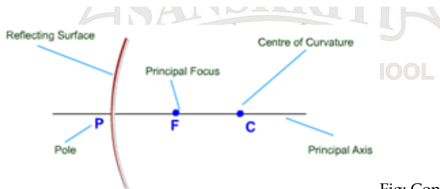
Fig: Convex Mirror
